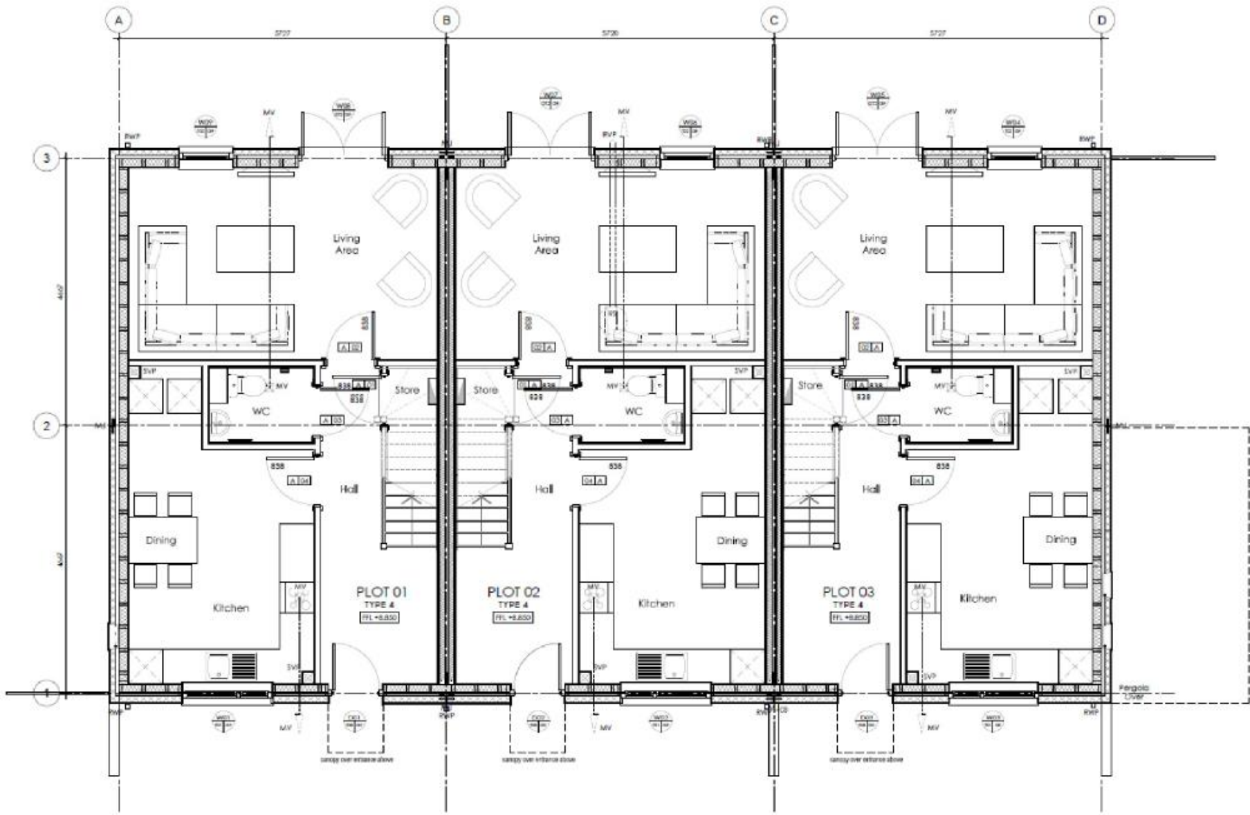
Ground Floor General Arrangement - Zone 1 - Plots 01-03
